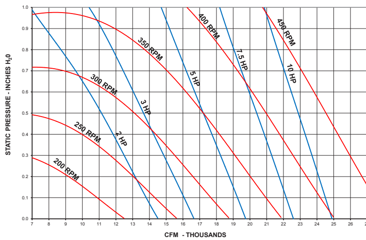
ID/IS/IUP800 w/ WS844 - Airflow Data
